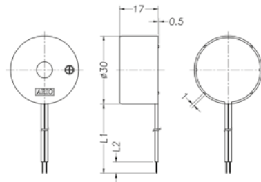
Lead Wire: UL 1095 AWG28 L1: 80 ± 5mm L2: 3 ± 1mm
