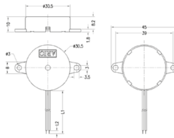
Lead Wire: UL 1095 AWG28 L1: 80 ± 5mm L2: 3.0 ± 1mm
