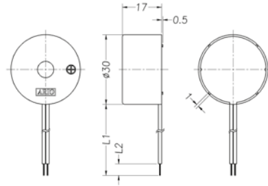
Lead Wire: UL 1095 AWG28 L1: 80 ± 5mm L2: 3.0 ± 1mm
